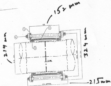
200 NB SINGLE SLEEVE COUPLING ASSY. (FOR ERW PIPE) ASSY. NO. SEE TABLE
