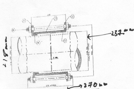
200 NB SINGLE SLEEVE COUPLING ASSY. (FOR ERW PIPE TO FITTING) ASSY. NO. SEE TABLE
