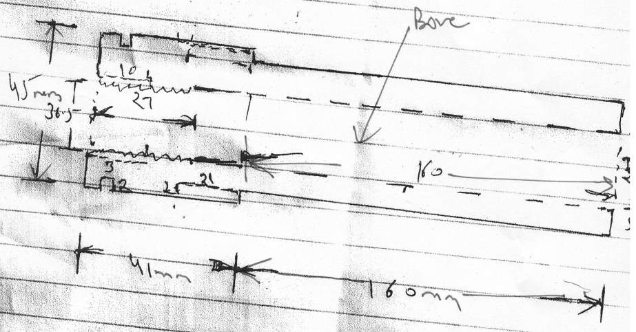
Ecc Pump shaft Sleeve
